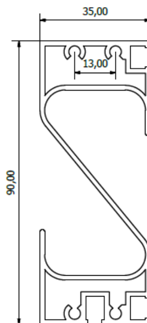
S-HANDGREEP
